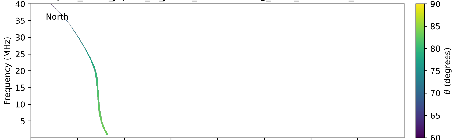
expres_earth_jupiter_io_jrm09_lossc-wid1deg_3kev_19770929_v11.cdf
