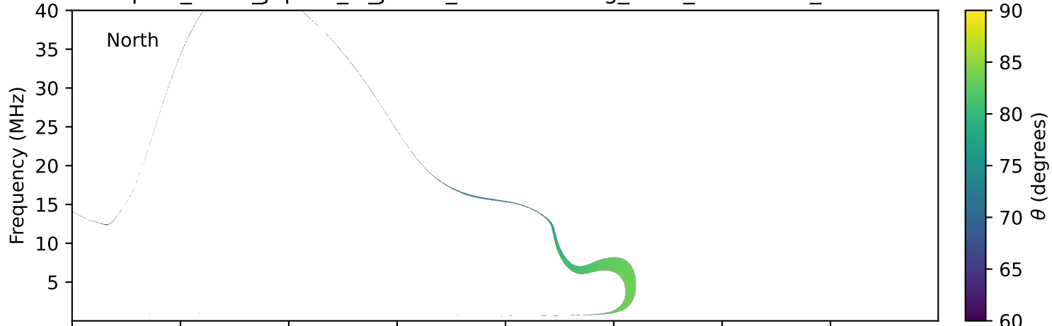
expres_earth_jupiter_io_jrm09_lossc-wid1deg_3kev_19770918_v11.cdf
