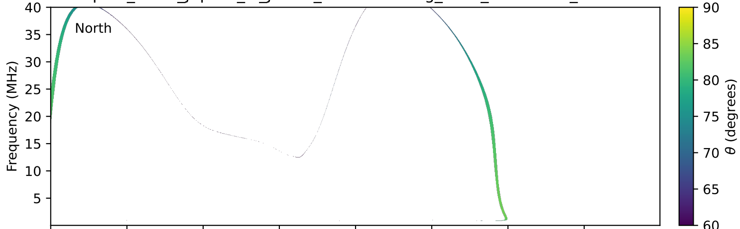
expres_earth_jupiter_io_jrm09_lossc-wid1deg_3kev_19770909_v11.cdf
