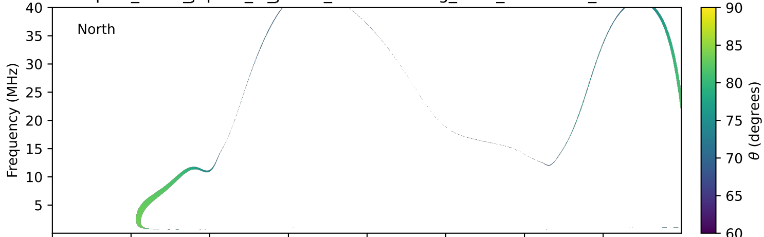
expres_earth_jupiter_io_jrm09_lossc-wid1deg_3kev_19770907_v11.cdf
