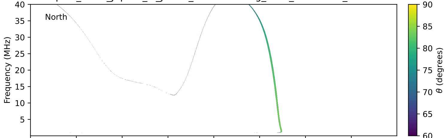
expres_earth_jupiter_io_jrm09_lossc-wid1deg_3kev_19770902_v11.cdf
