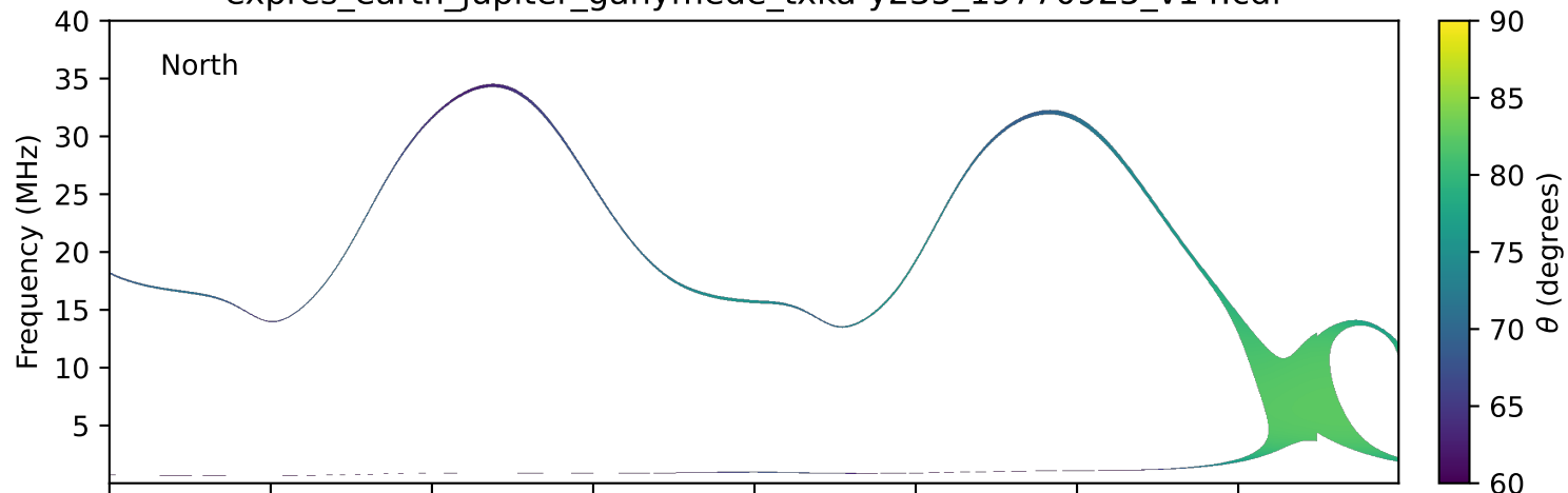
expres_earth_jupiter_ganymede_txka-y235_19770925_v14.cdf
