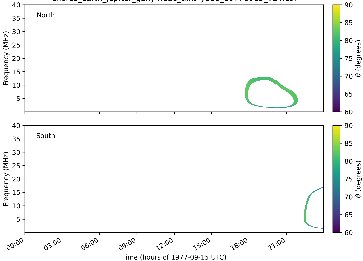
expres_earth_jupiter_ganymede_txka-y235_19770915_v14.cdf
