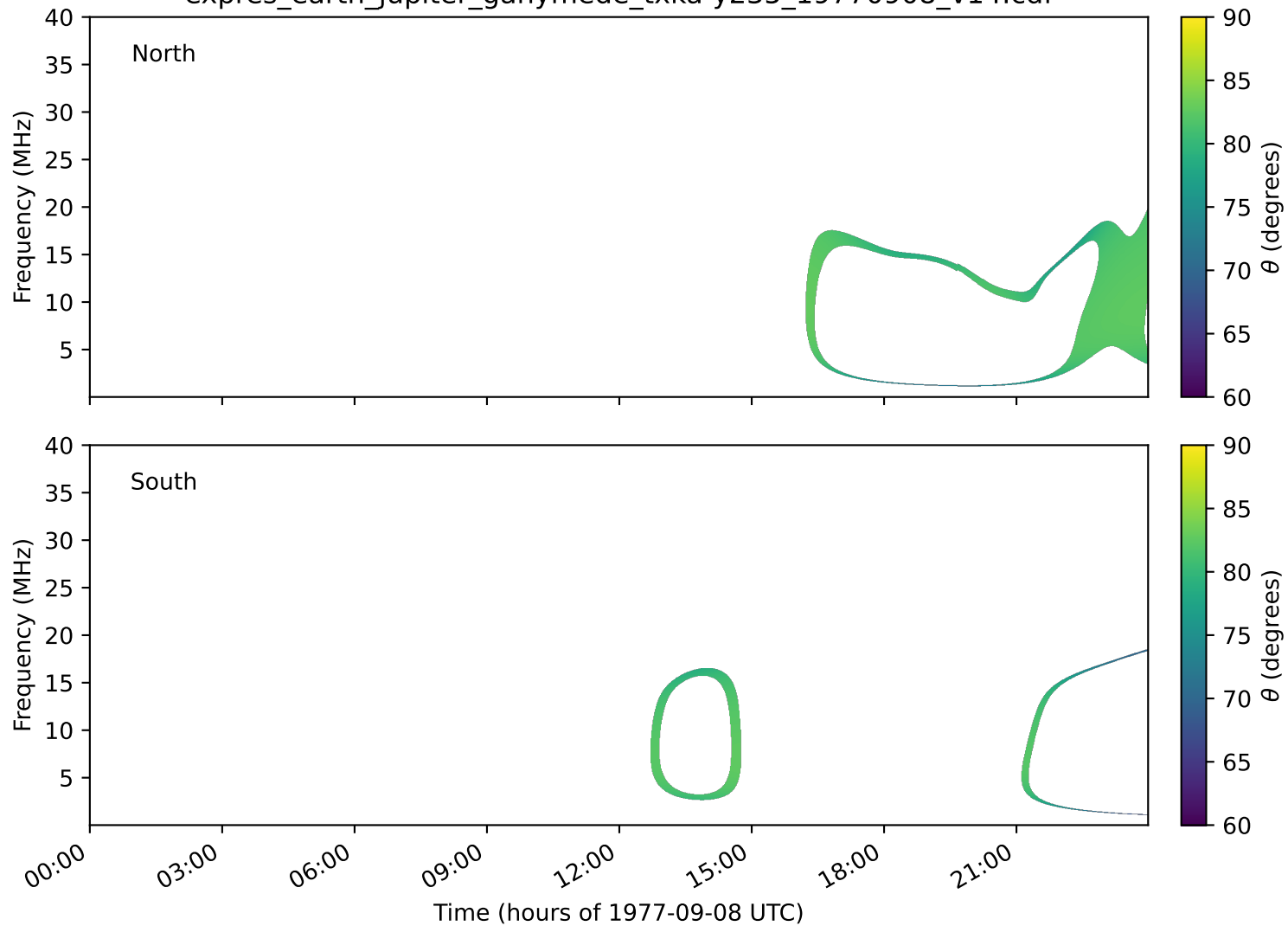
expres_earth_jupiter_ganymede_txka-y235_19770908_v14.cdf
