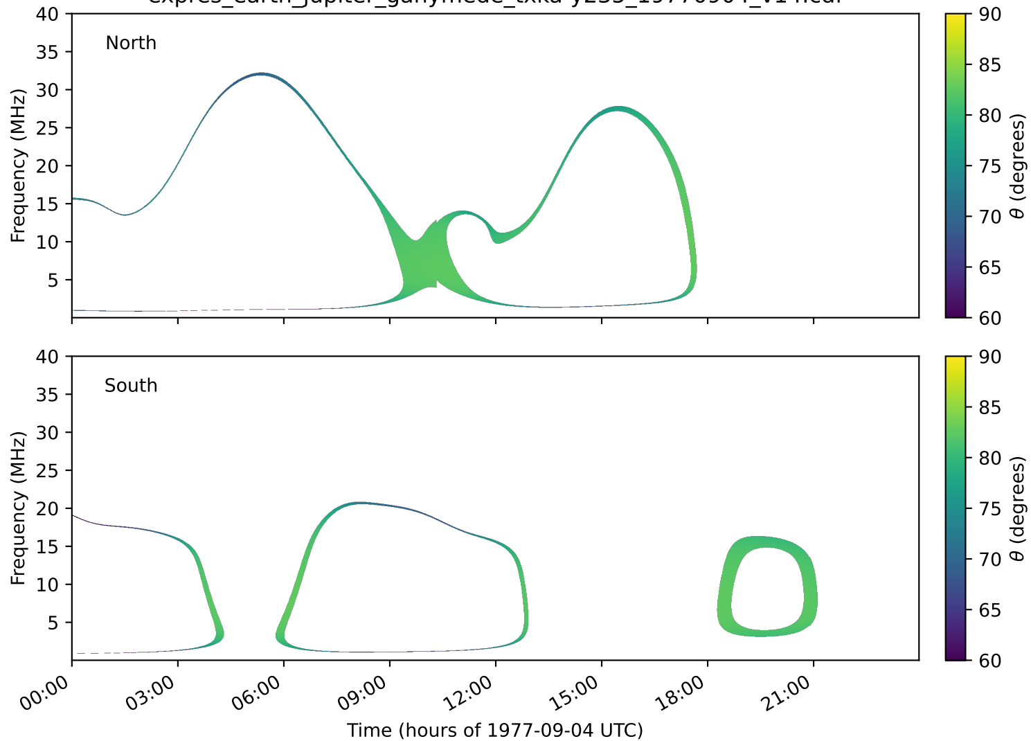
expres_earth_jupiter_ganymede_txka-y235_19770904_v14.cdf
