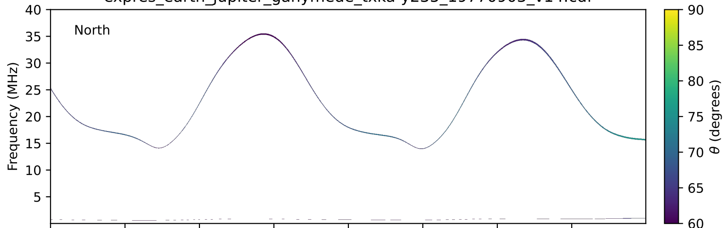
expres_earth_jupiter_ganymede_txka-y235_19770903_v14.cdf
