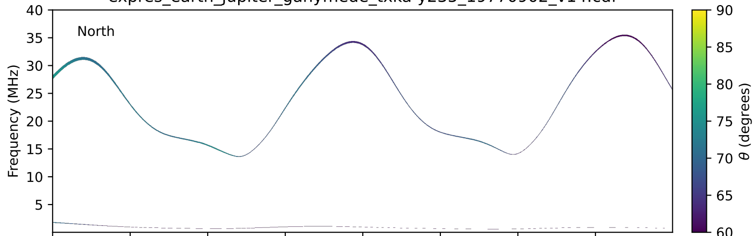
expres_earth_jupiter_ganymede_txka-y235_19770902_v14.cdf
