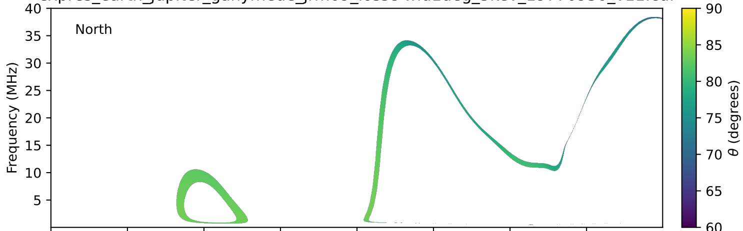
expres_earth_jupiter_ganymede_jrm09_lossc-wid1deg_3kev_19770930_v11.cdf
