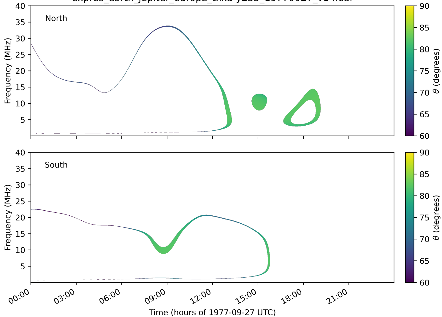
expres_earth_jupiter_europa_txka-y235_19770927_v14.cdf
