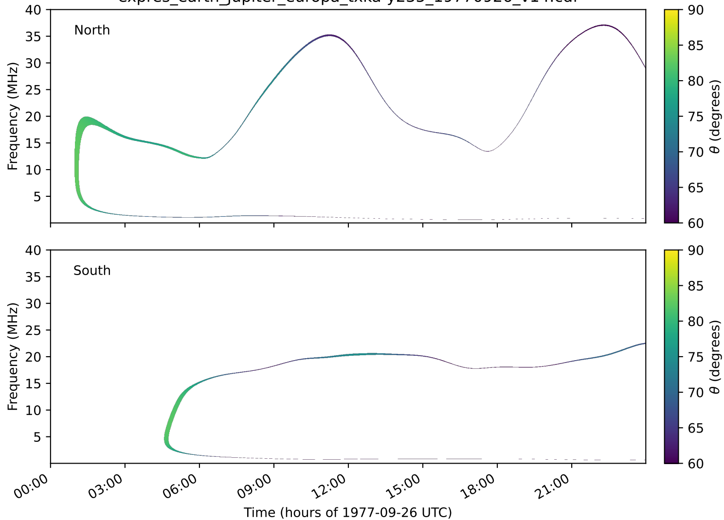
expres_earth_jupiter_europa_txka-y235_19770926_v14.cdf
