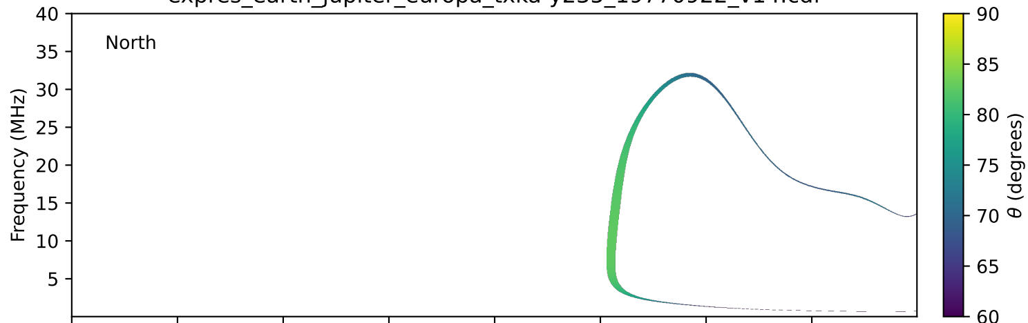
expres_earth_jupiter_europa_txka-y235_19770922_v14.cdf
