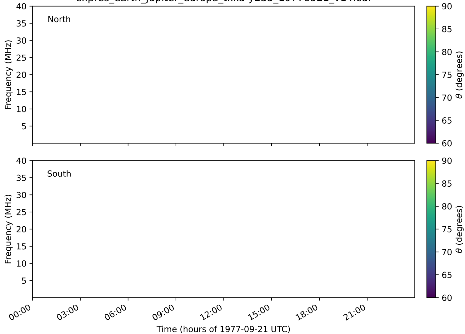
expres_earth_jupiter_europa_txka-y235_19770921_v14.cdf
