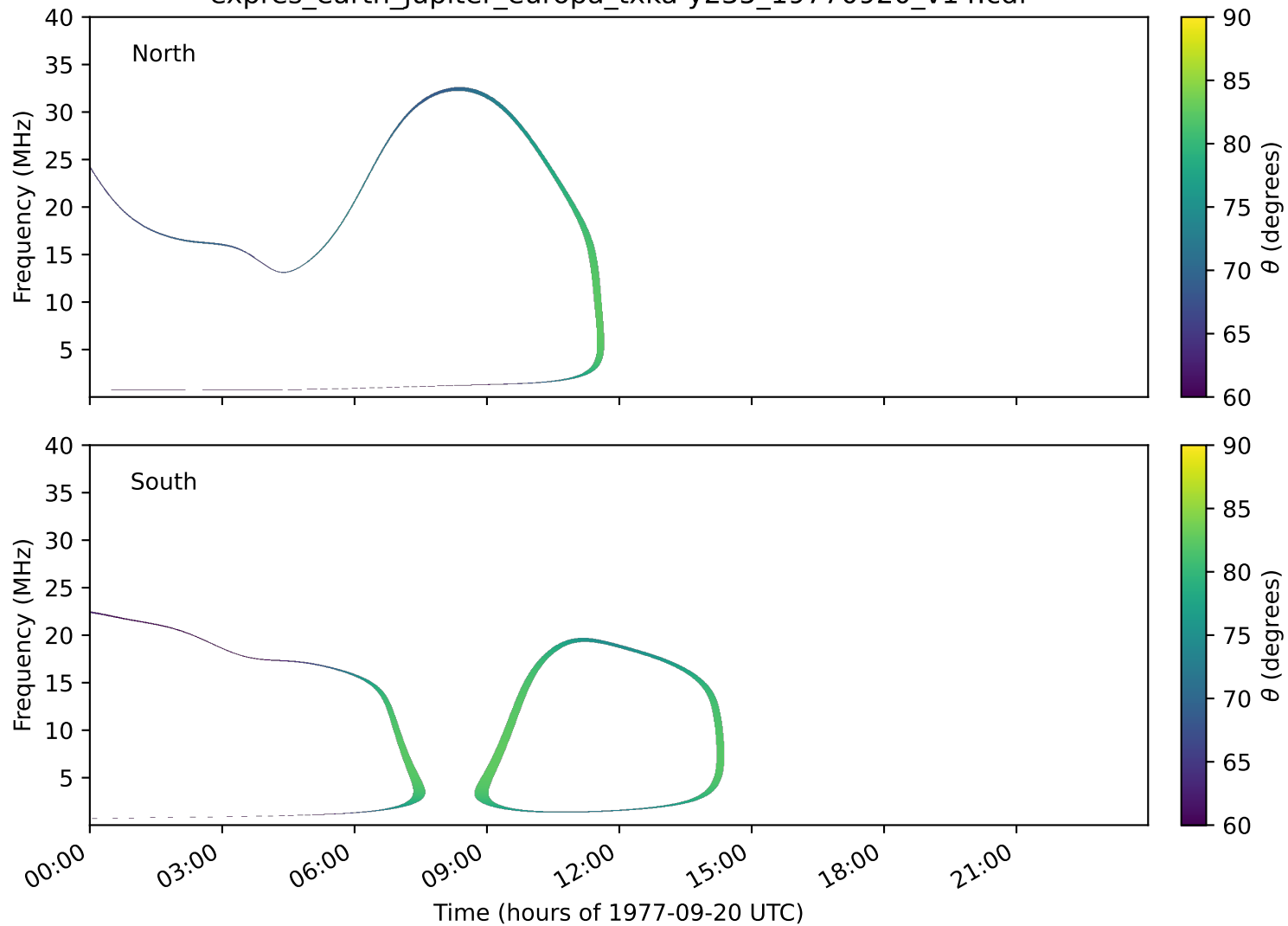
expres_earth_jupiter_europa_txka-y235_19770920_v14.cdf
