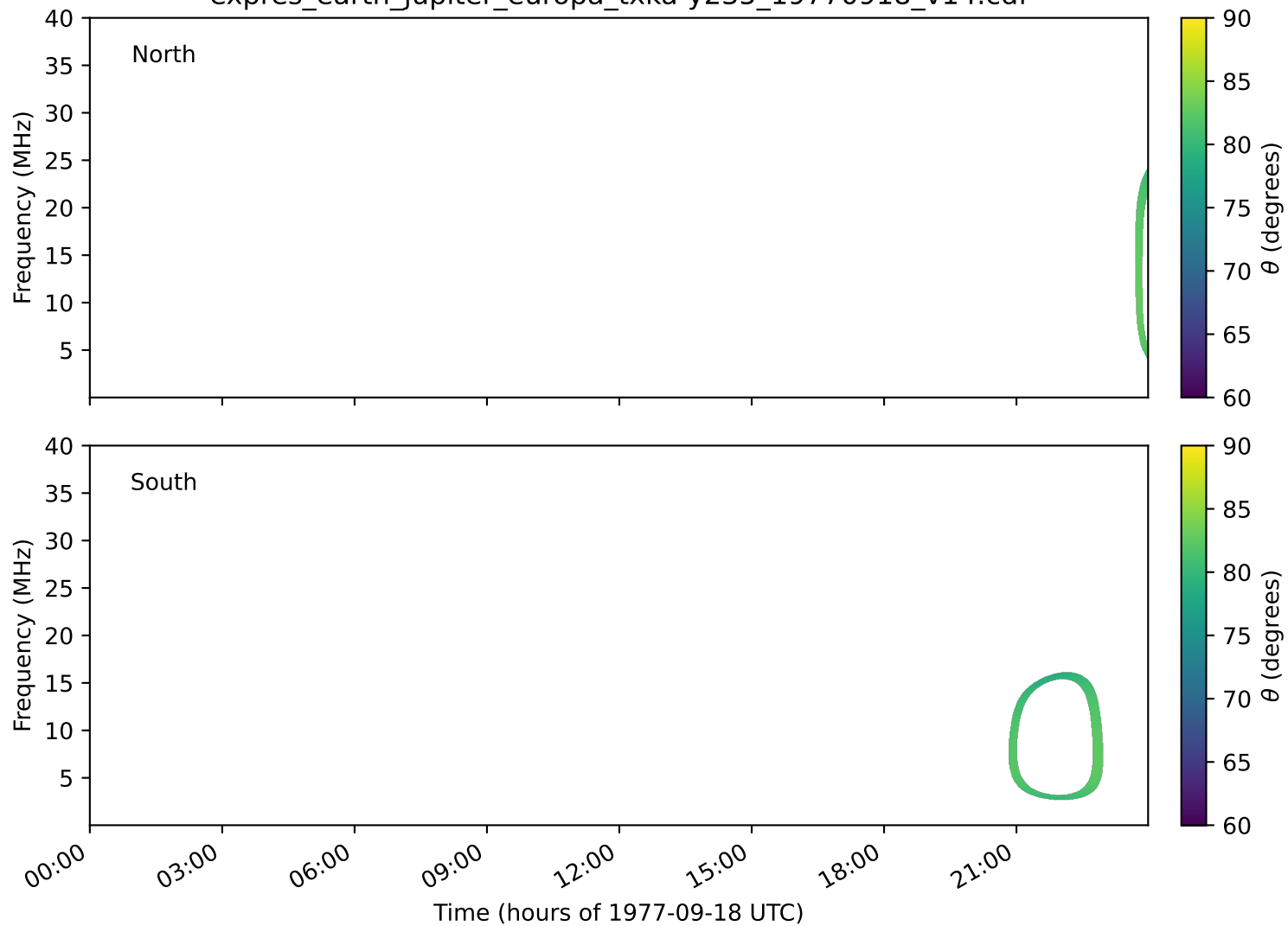
expres_earth_jupiter_europa_txka-y235_19770918_v14.cdf
