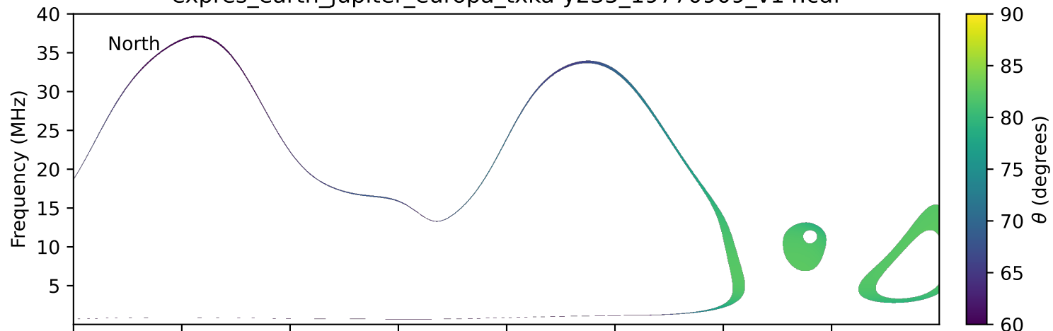
expres_earth_jupiter_europa_txka-y235_19770909_v14.cdf
