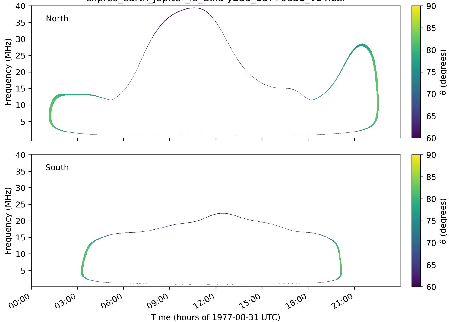
expres_earth_jupiter_io_txka-y235_19770831_v14.cdf
