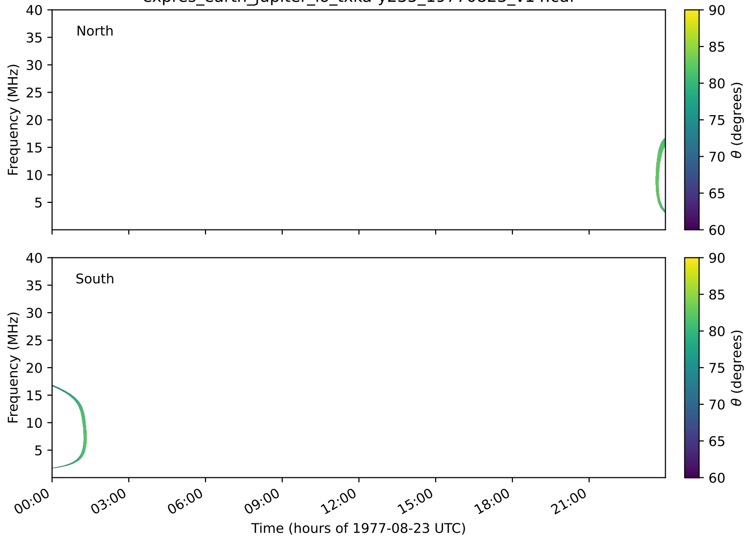
expres_earth_jupiter_io_txka-y235_19770823_v14.cdf
