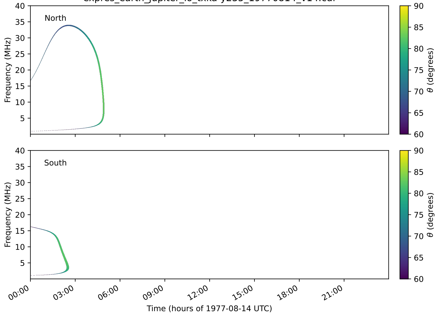
expres_earth_jupiter_io_txka-y235_19770814_v14.cdf
