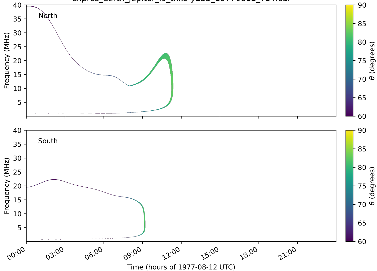
expres_earth_jupiter_io_txka-y235_19770812_v14.cdf
