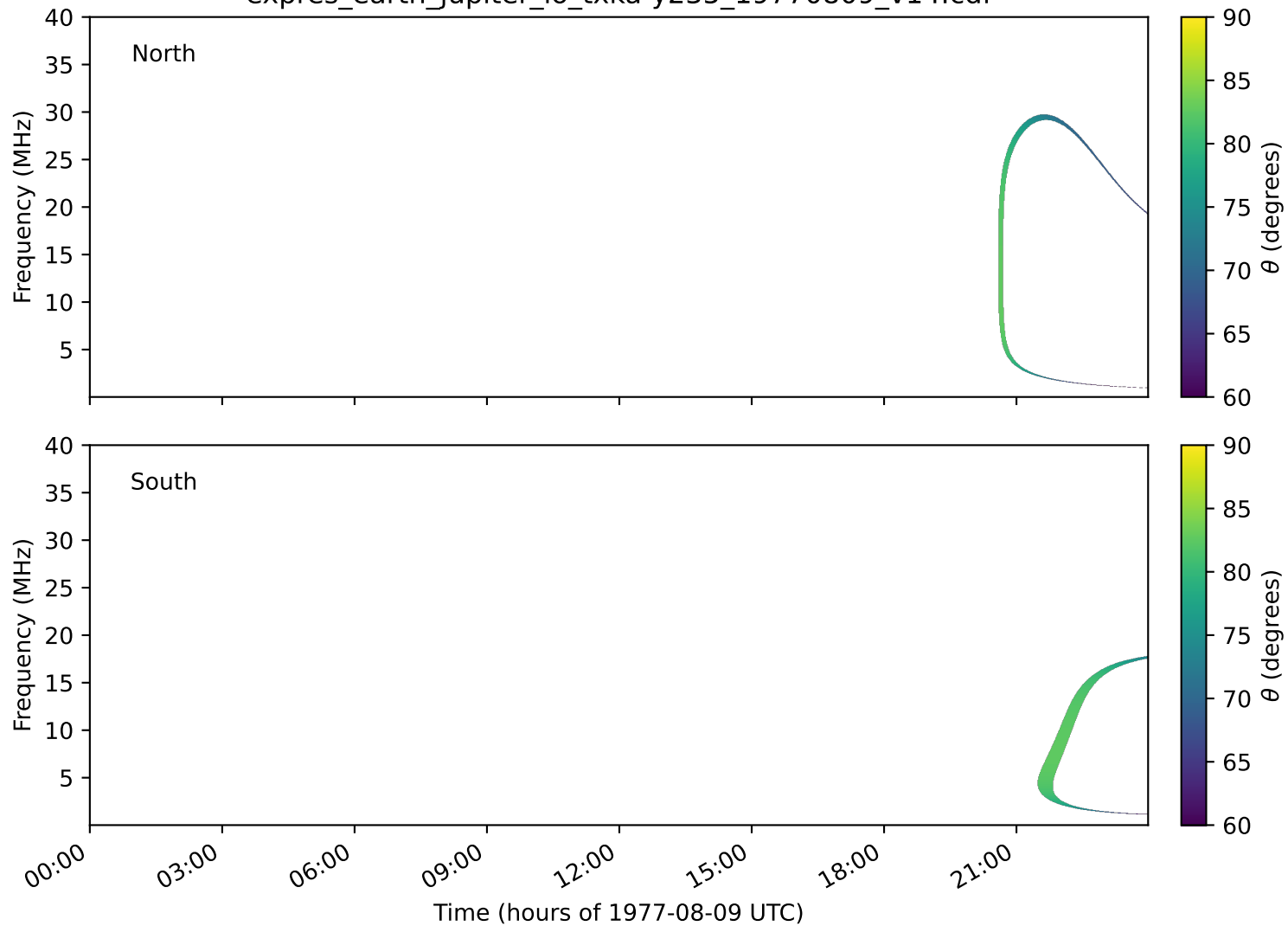
expres_earth_jupiter_io_txka-y235_19770809_v14.cdf
