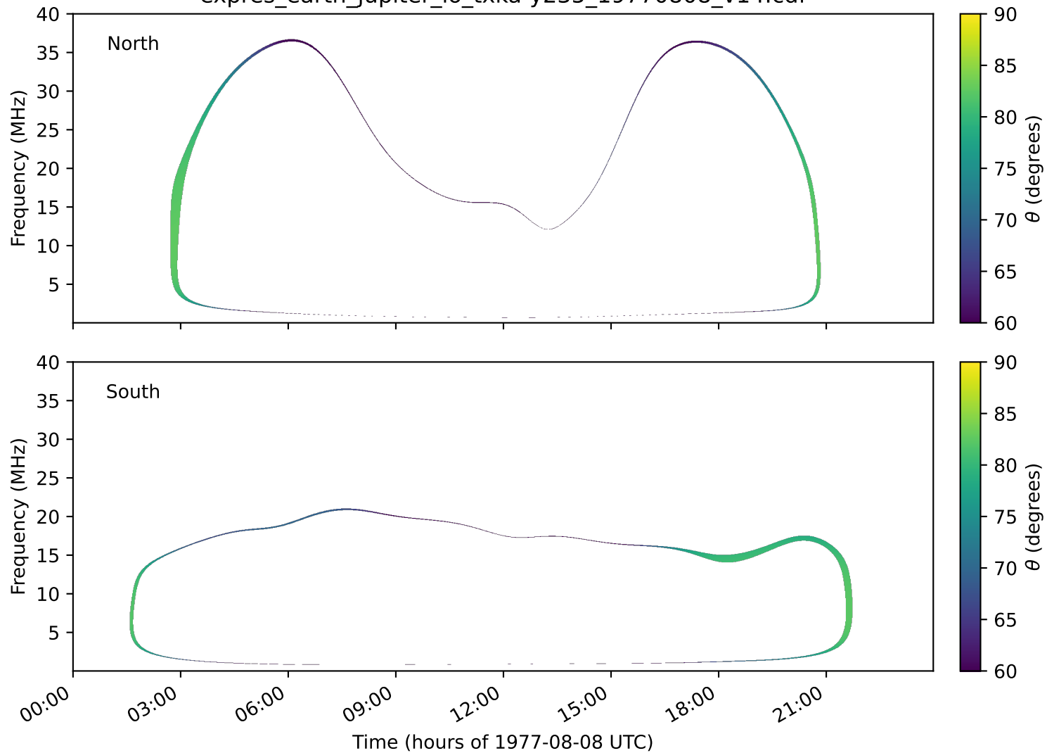
expres_earth_jupiter_io_txka-y235_19770808_v14.cdf
