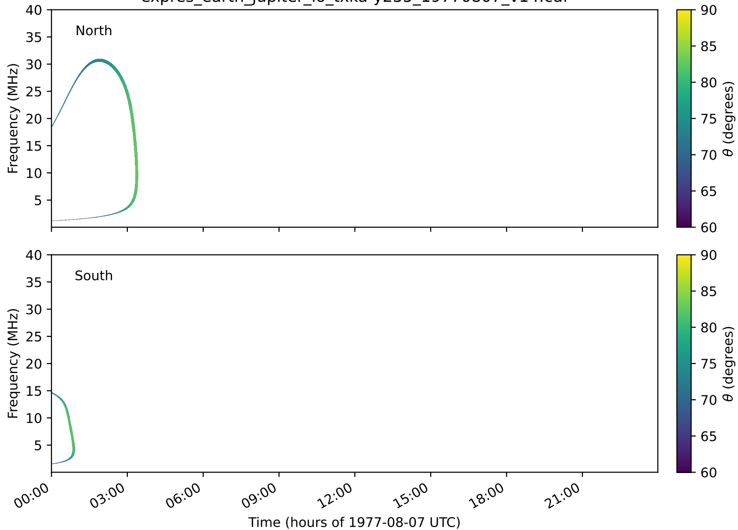
expres_earth_jupiter_io_txka-y235_19770807_v14.cdf
