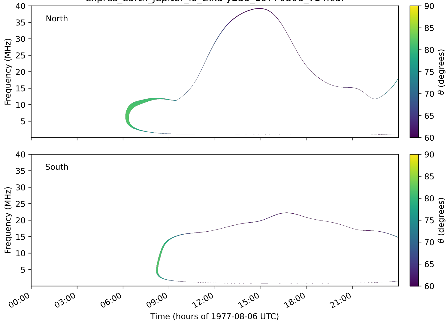
expres_earth_jupiter_io_txka-y235_19770806_v14.cdf
