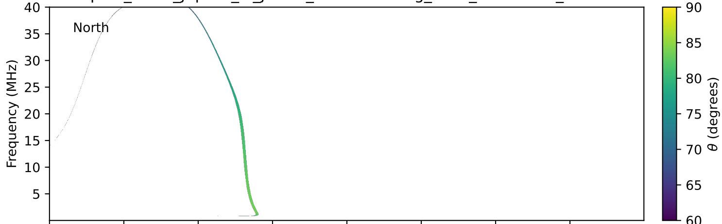
expres_earth_jupiter_io_jrm33_lossc-wid1deg_3kev_19770828_v11.cdf
