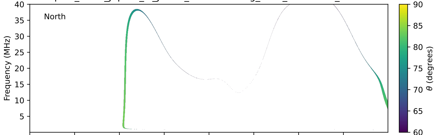
expres_earth_jupiter_io_jrm33_lossc-wid1deg_3kev_19770822_v11.cdf
