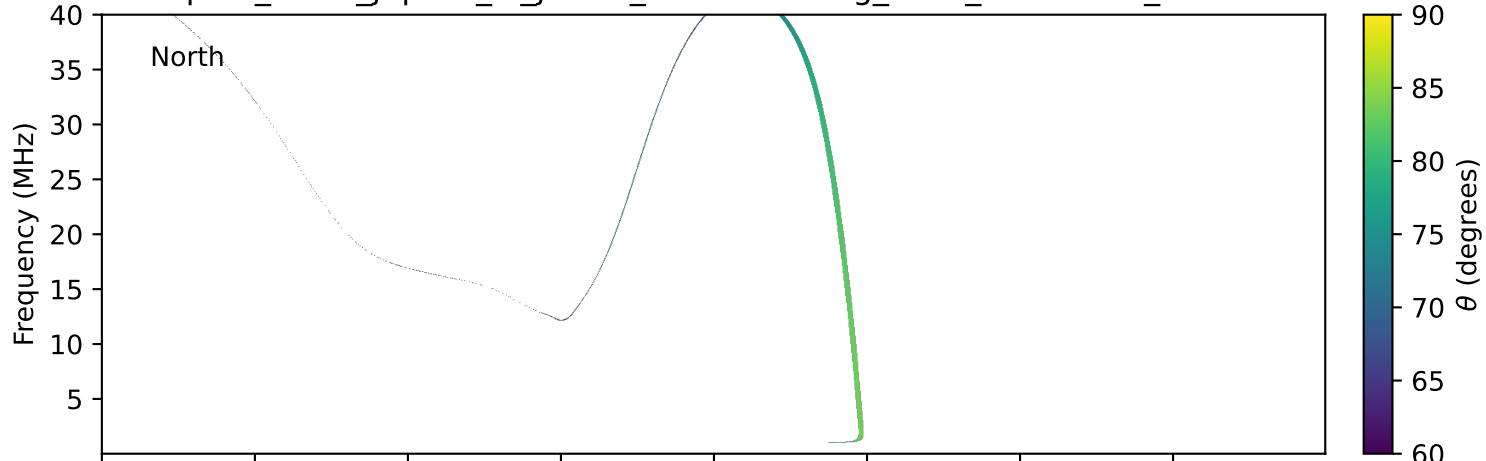
expres_earth_jupiter_io_jrm09_lossc-wid1deg_3kev_19770826_v11.cdf
