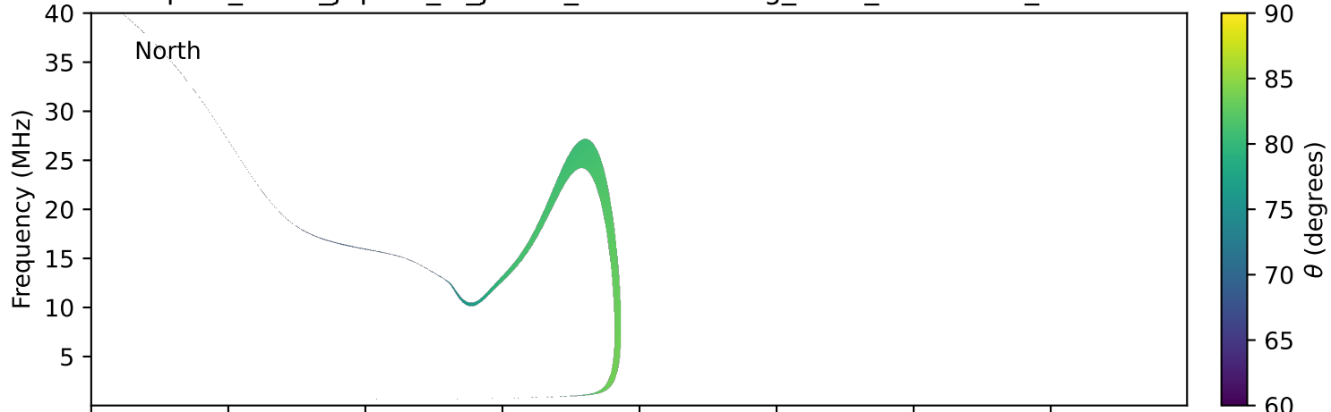
expres_earth_jupiter_io_jrm09_lossc-wid1deg_3kev_19770812_v11.cdf
