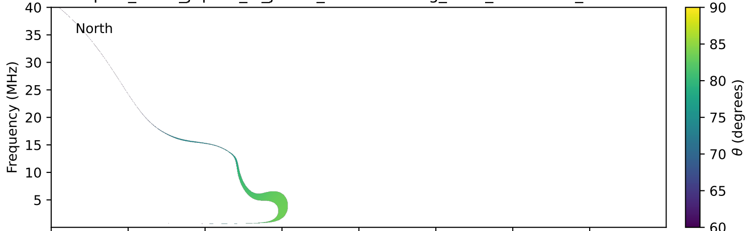
expres_earth_jupiter_io_jrm09_lossc-wid1deg_3kev_19770805_v11.cdf
