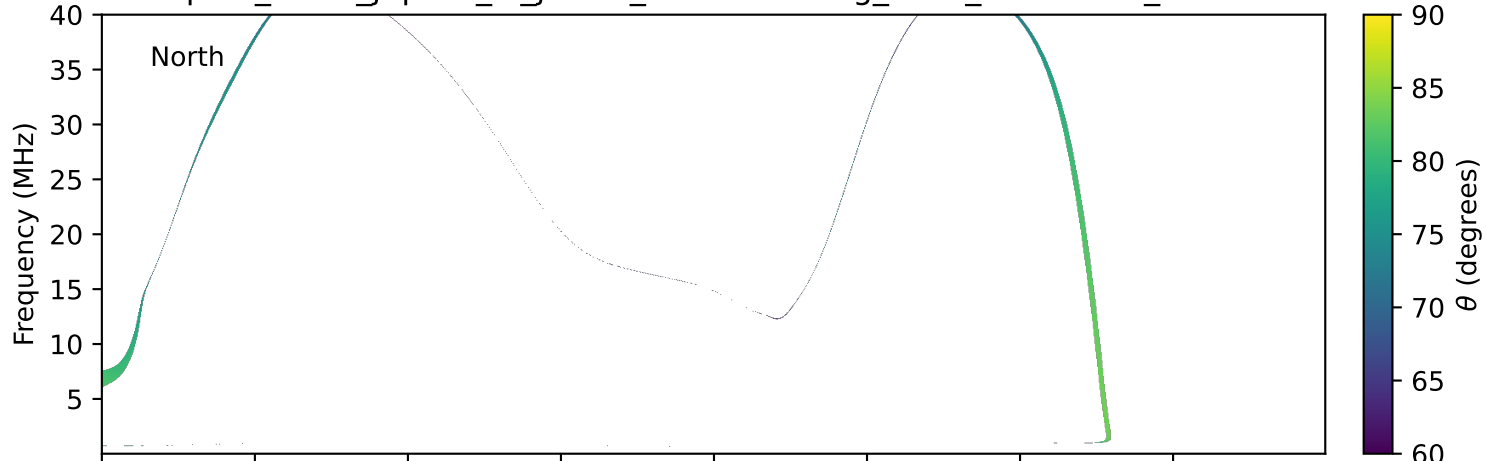
expres_earth_jupiter_io_jrm09_lossc-wid1deg_3kev_19770801_v11.cdf
