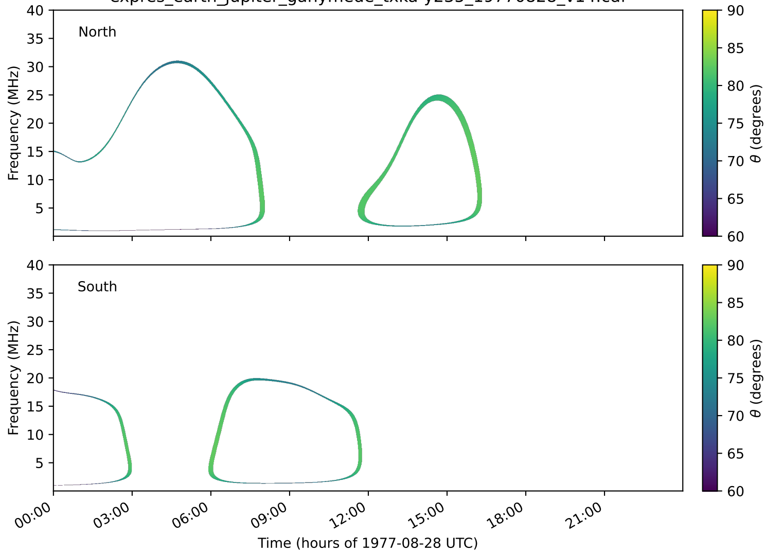
expres_earth_jupiter_ganymede_txka-y235_19770828_v14.cdf
