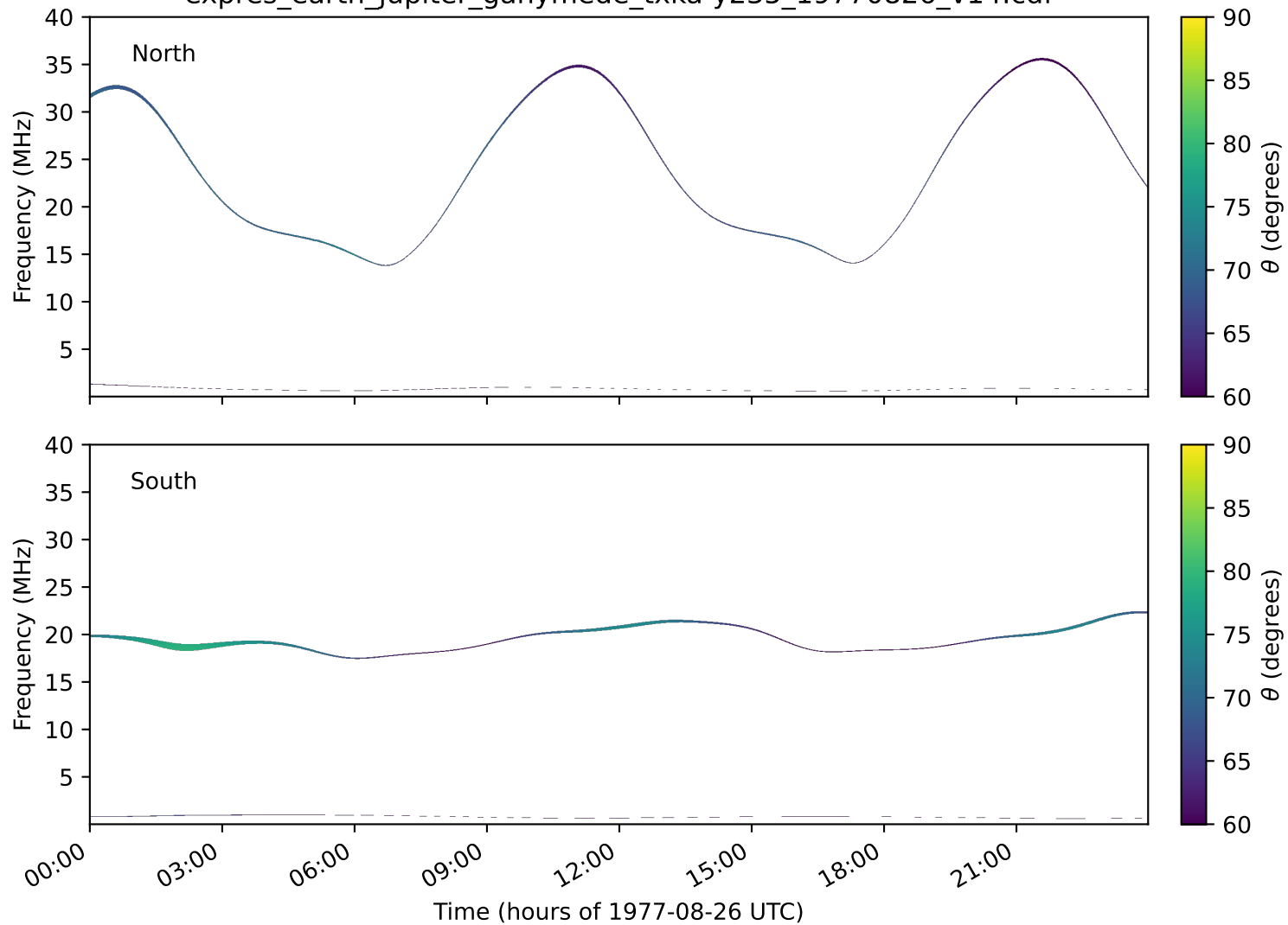
expres_earth_jupiter_ganymede_txka-y235_19770826_v14.cdf
