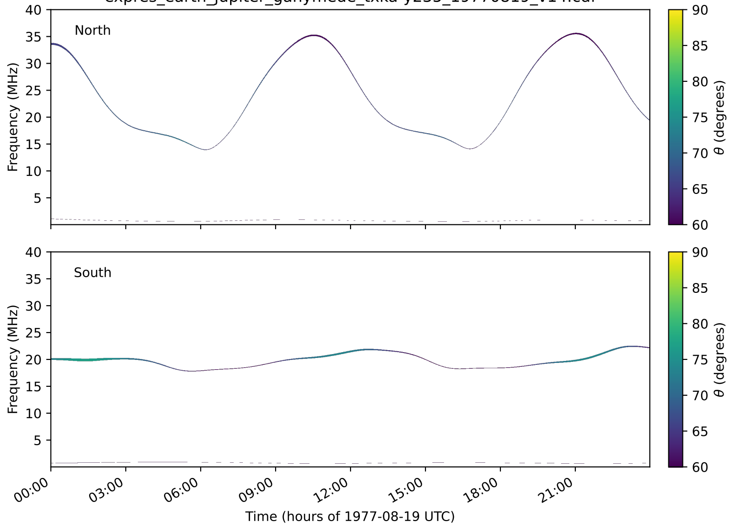
expres_earth_jupiter_ganymede_txka-y235_19770819_v14.cdf
