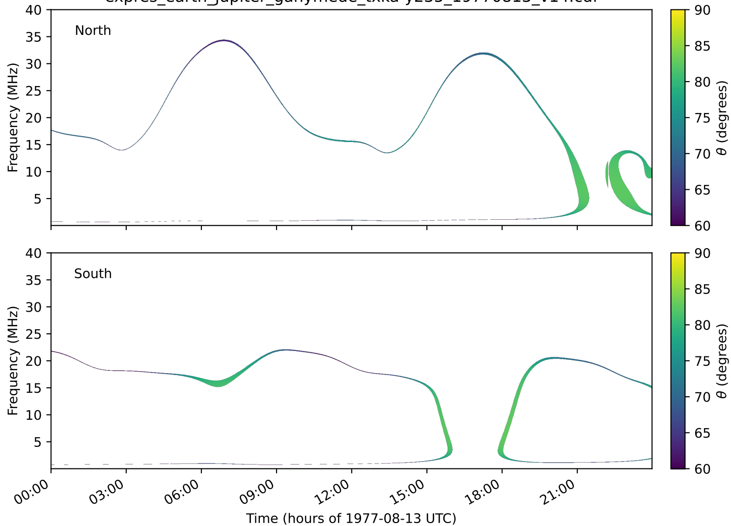
expres_earth_jupiter_ganymede_txka-y235_19770813_v14.cdf
