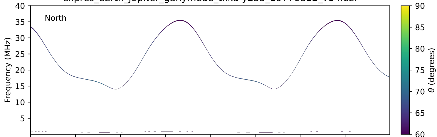
expres_earth_jupiter_ganymede_txka-y235_19770812_v14.cdf
