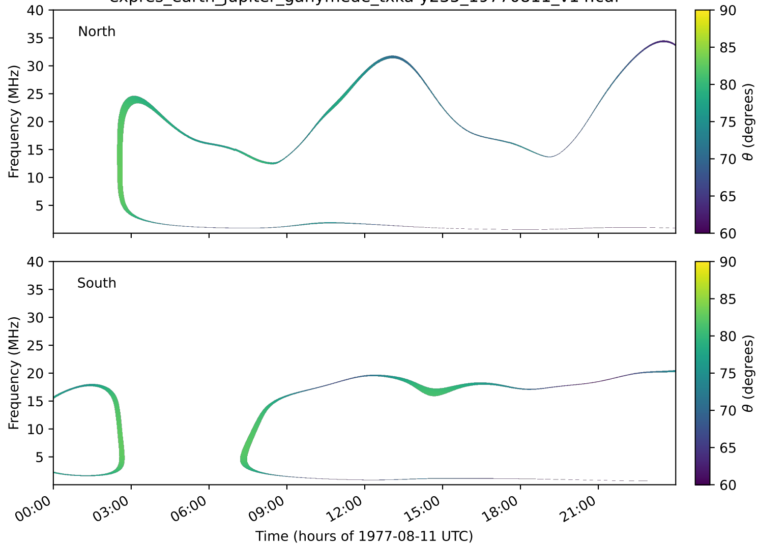
expres_earth_jupiter_ganymede_txka-y235_19770811_v14.cdf
