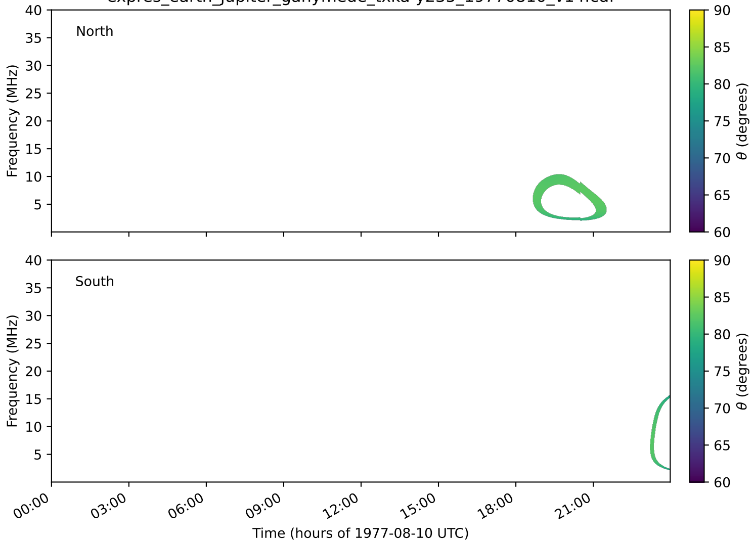
expres_earth_jupiter_ganymede_txka-y235_19770810_v14.cdf
