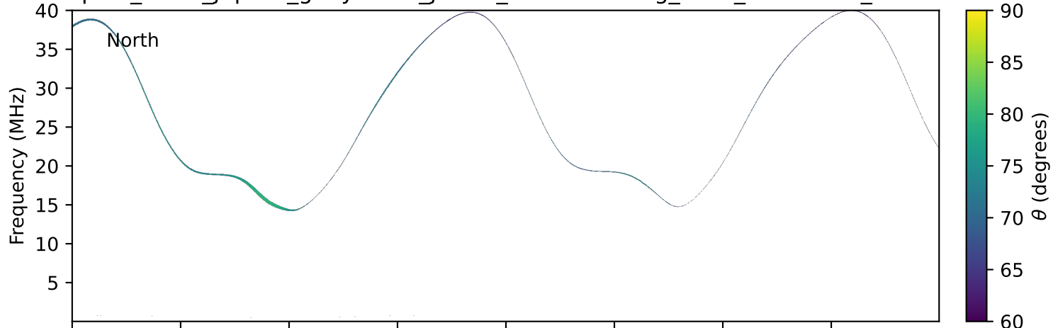
expres_earth_jupiter_ganymede_jrm33_lossc-wid1deg_3kev_19770826_v11.cdf
