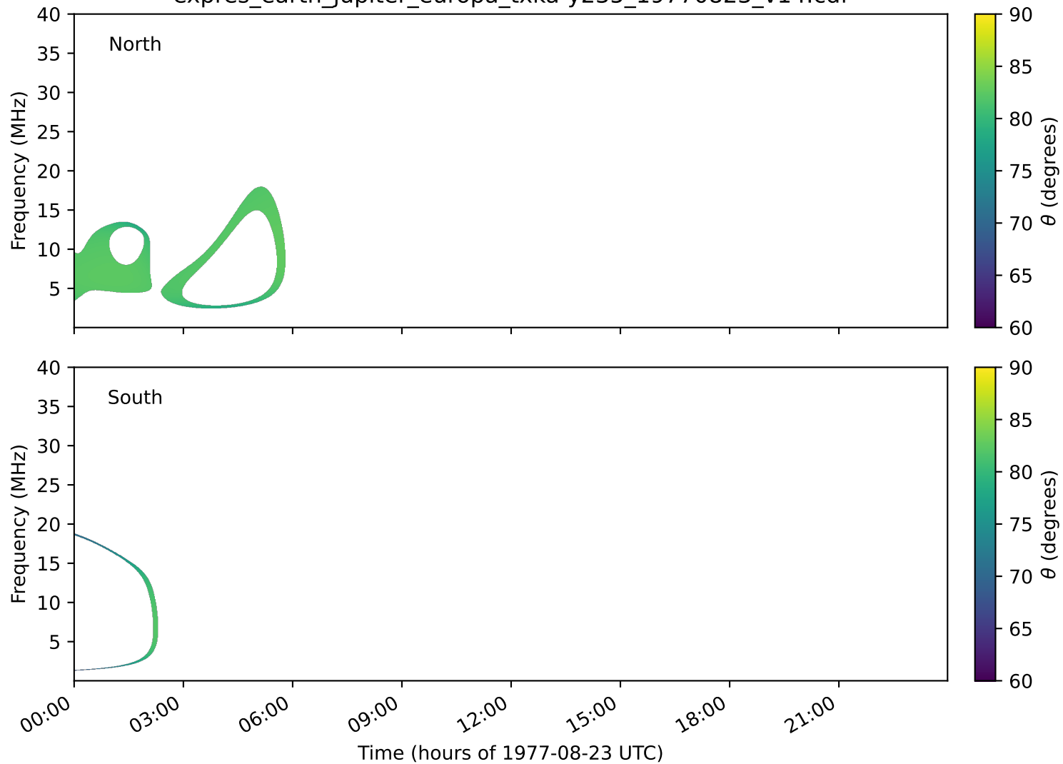
expres_earth_jupiter_europa_txka-y235_19770823_v14.cdf
