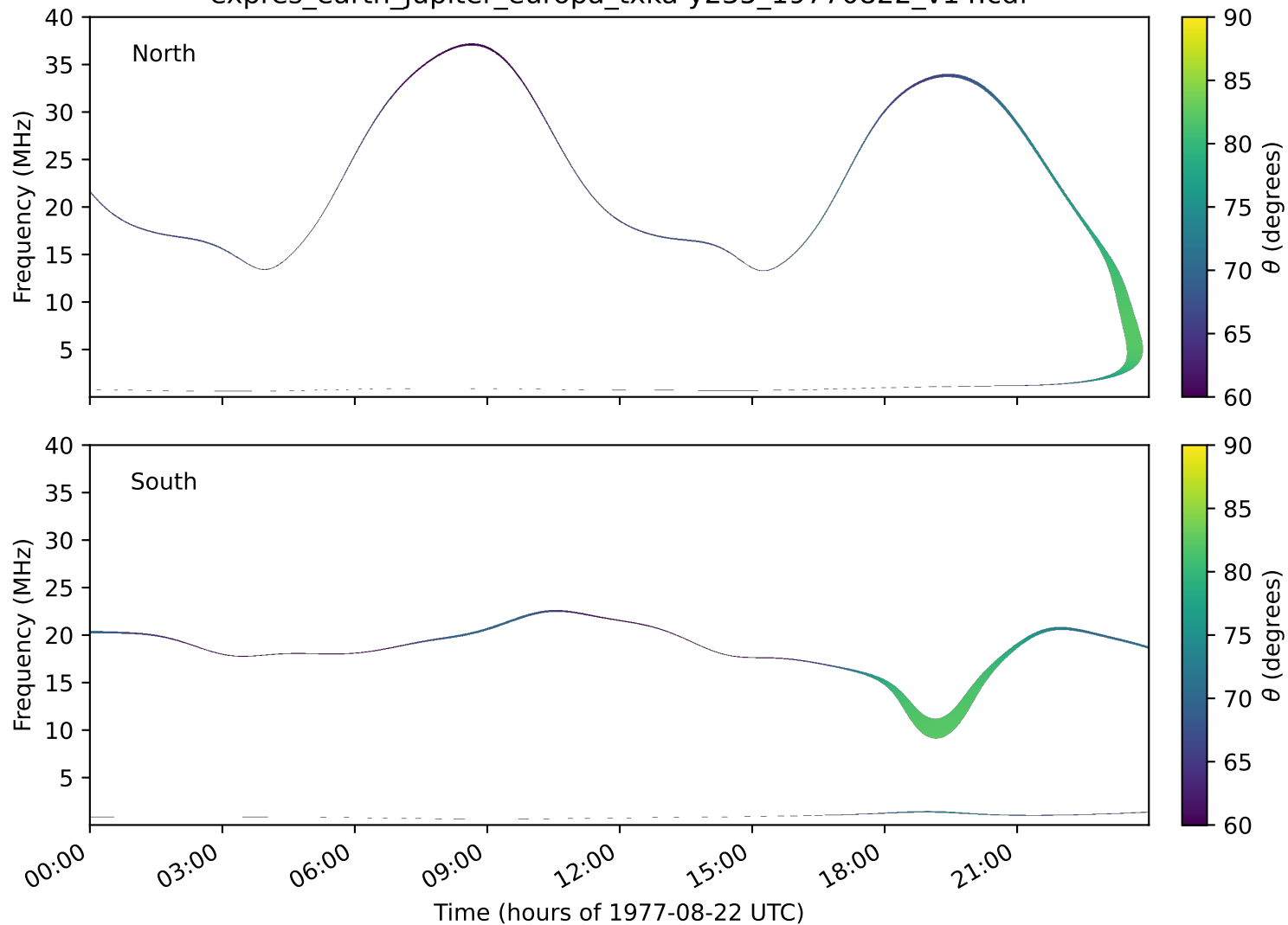
expres_earth_jupiter_europa_txka-y235_19770822_v14.cdf
