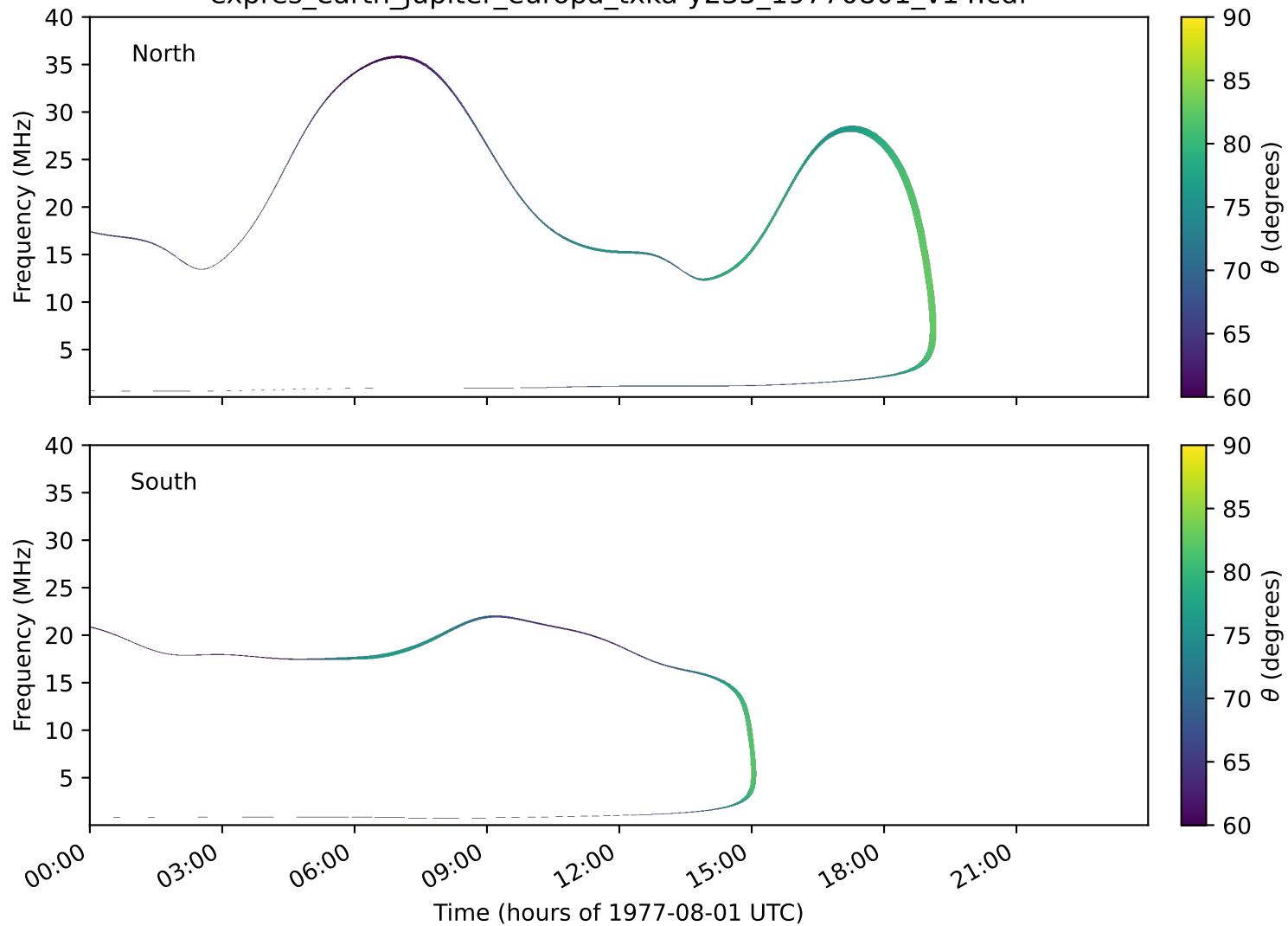
expres_earth_jupiter_europa_txka-y235_19770801_v14.cdf
