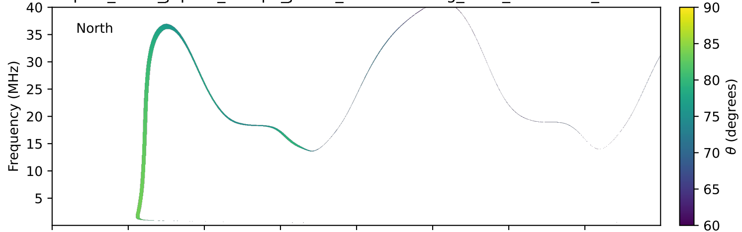
expres_earth_jupiter_europa_jrm33_lossc-wid1deg_3kev_19770825_v11.cdf
