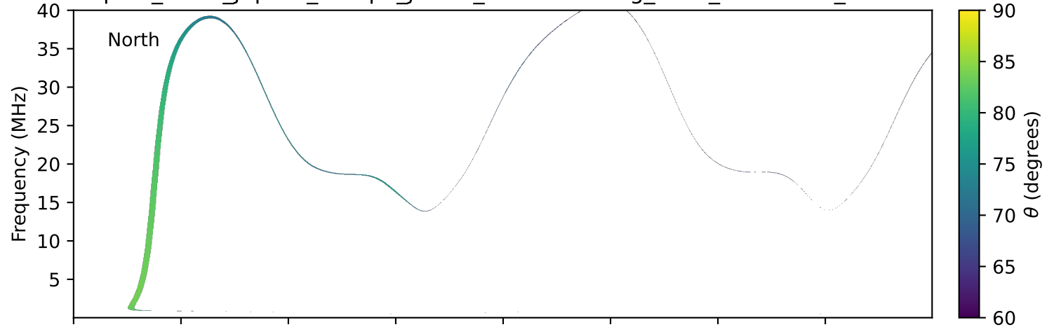
expres_earth_jupiter_europa_jrm33_lossc-wid1deg_3kev_19770818_v11.cdf
