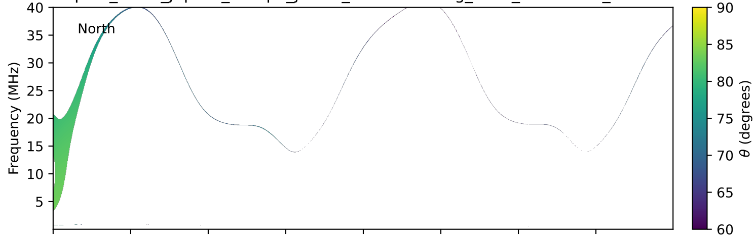
expres_earth_jupiter_europa_jrm33_lossc-wid1deg_3kev_19770811_v11.cdf
