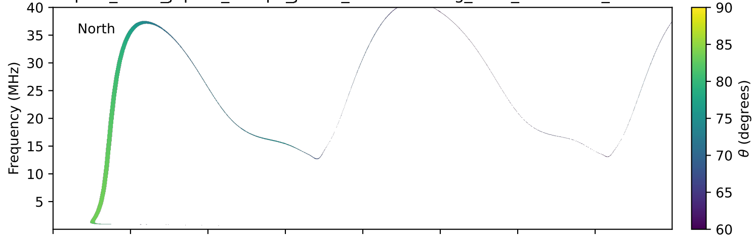
expres_earth_jupiter_europa_jrm09_lossc-wid1deg_3kev_19770818_v11.cdf
