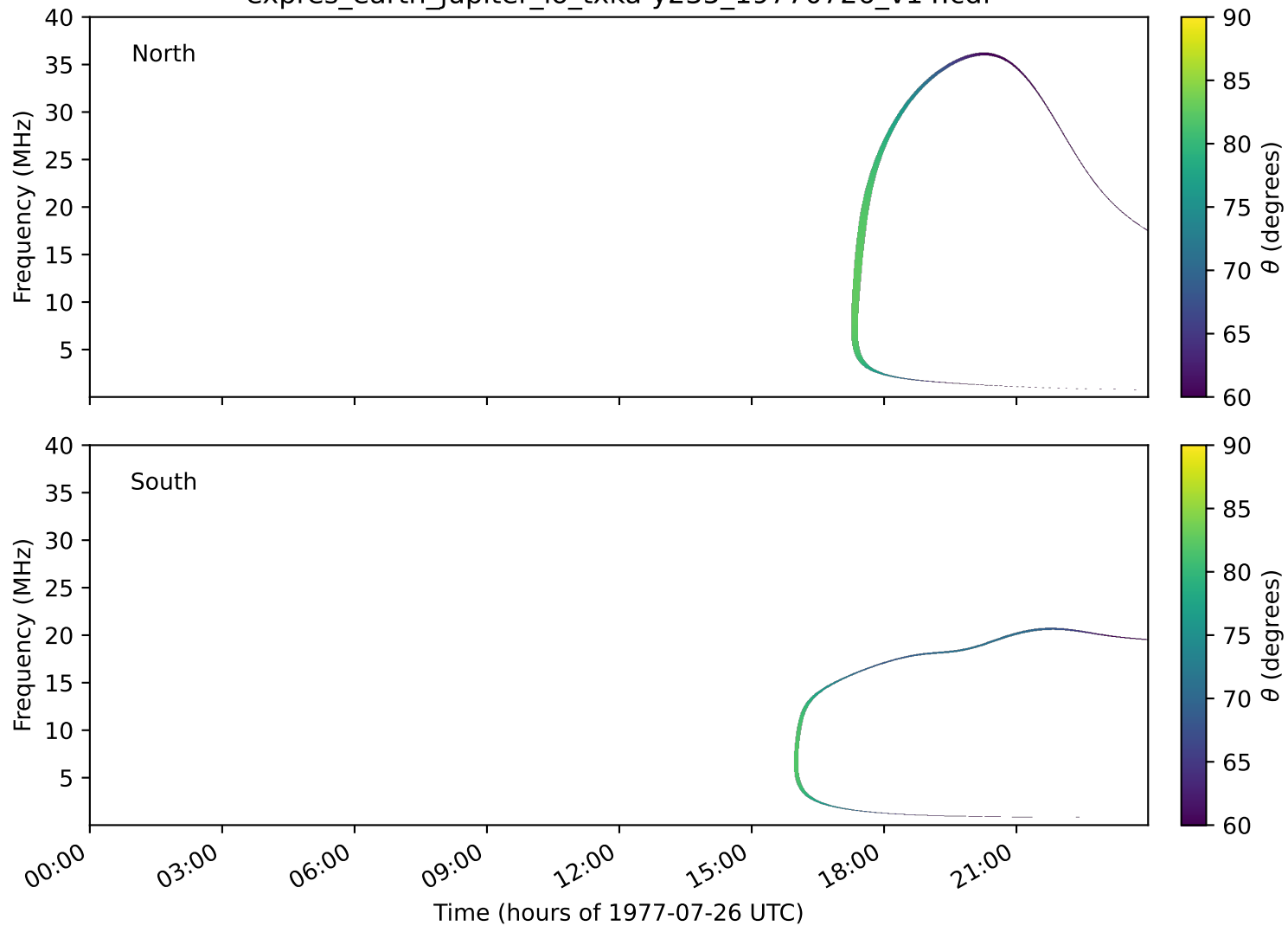
expres_earth_jupiter_io_txka-y235_19770726_v14.cdf
