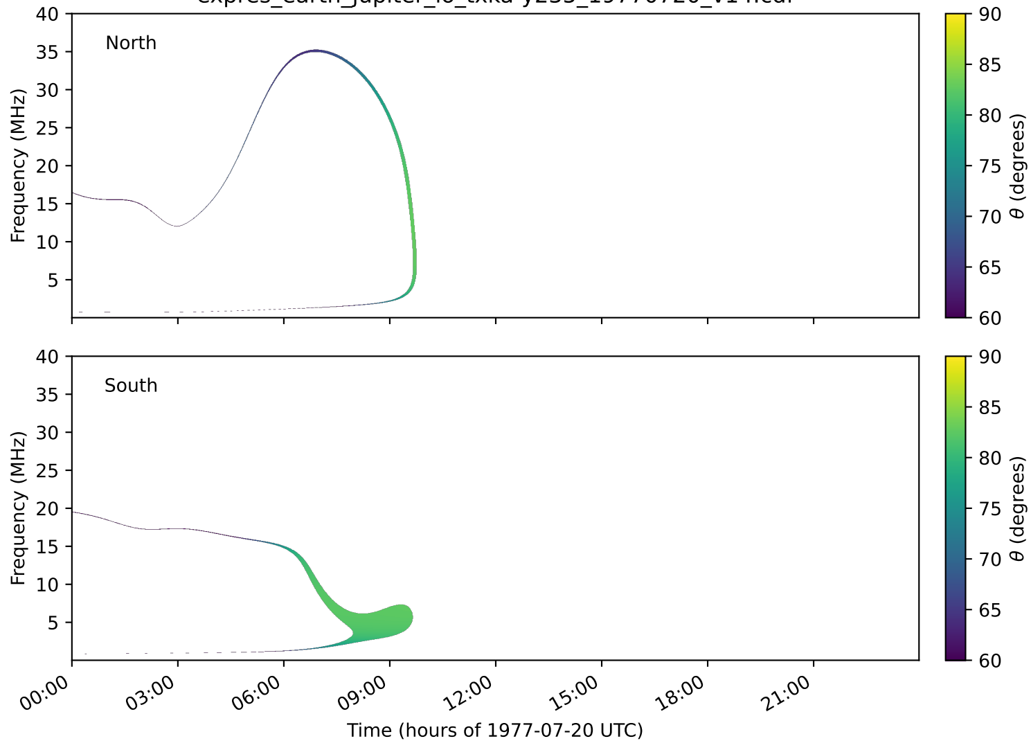
expres_earth_jupiter_io_txka-y235_19770720_v14.cdf
